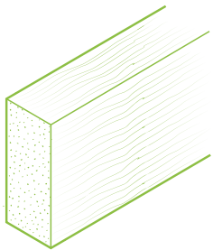
Horizontal Battens 58mm x 28mm
